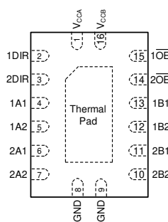
Figure 5-2. BQB/WBQB Package 16-Pin WQFN Transparent Top View
