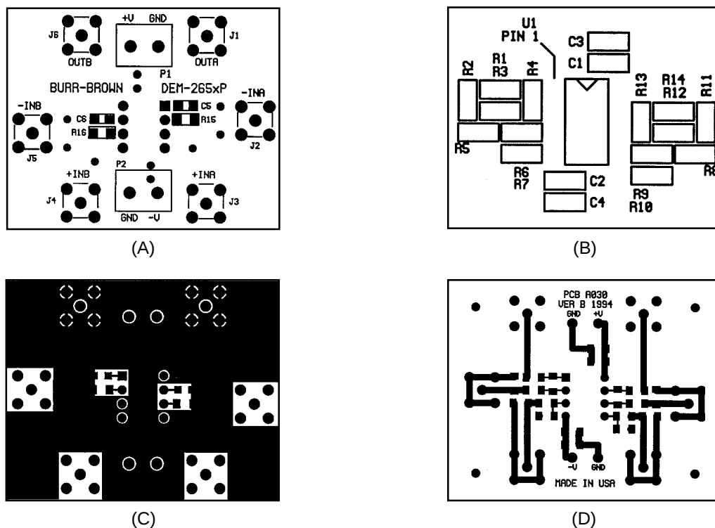
FIGURE 9. Evaluation Board Silkscreen (Solder Side). 9b. Evaluation Board Silkscreen (Component Side). 9c. Evaluation Board Layout (Solder Side). 9d. Evaluation Board (Component Side).
