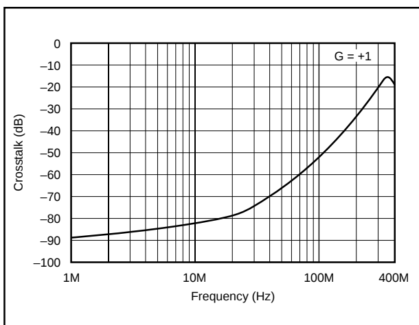
FIGURE 6. Channel-to-Channel Crosstalk.
