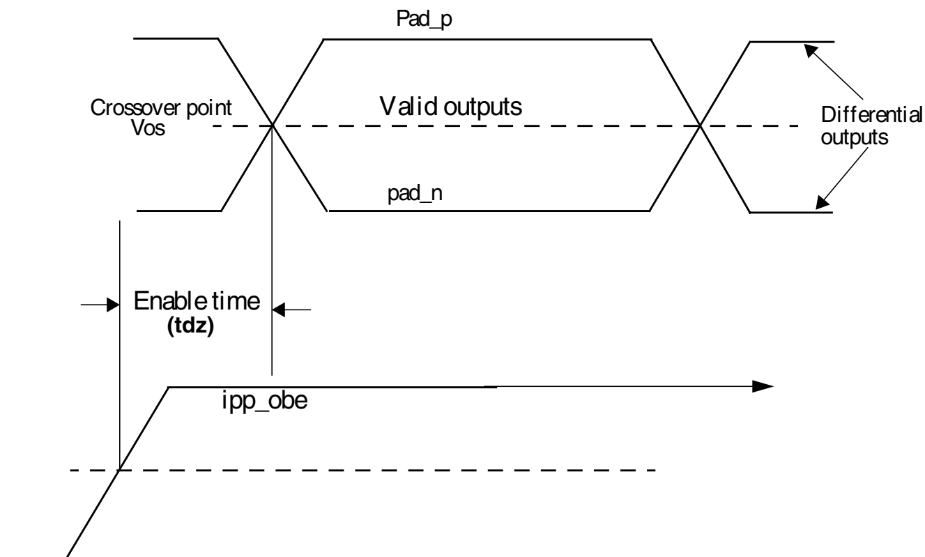
Figure 6. Enable time
