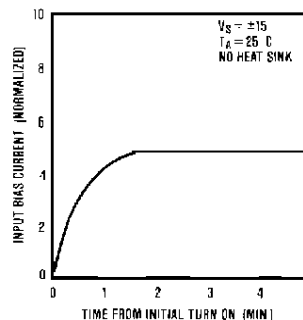
INPUT BIAS CURRENT AFTER WARM-UP
