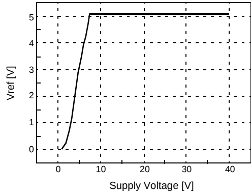
Figure 22. Reference Voltage
