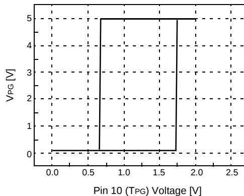
Figure 20. Hysteresis Voltage 2
