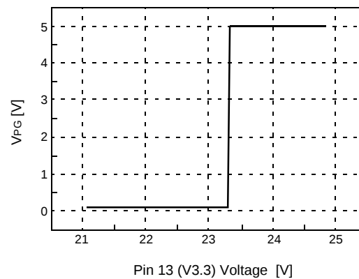
Figure 10. UVP for 3.3V
