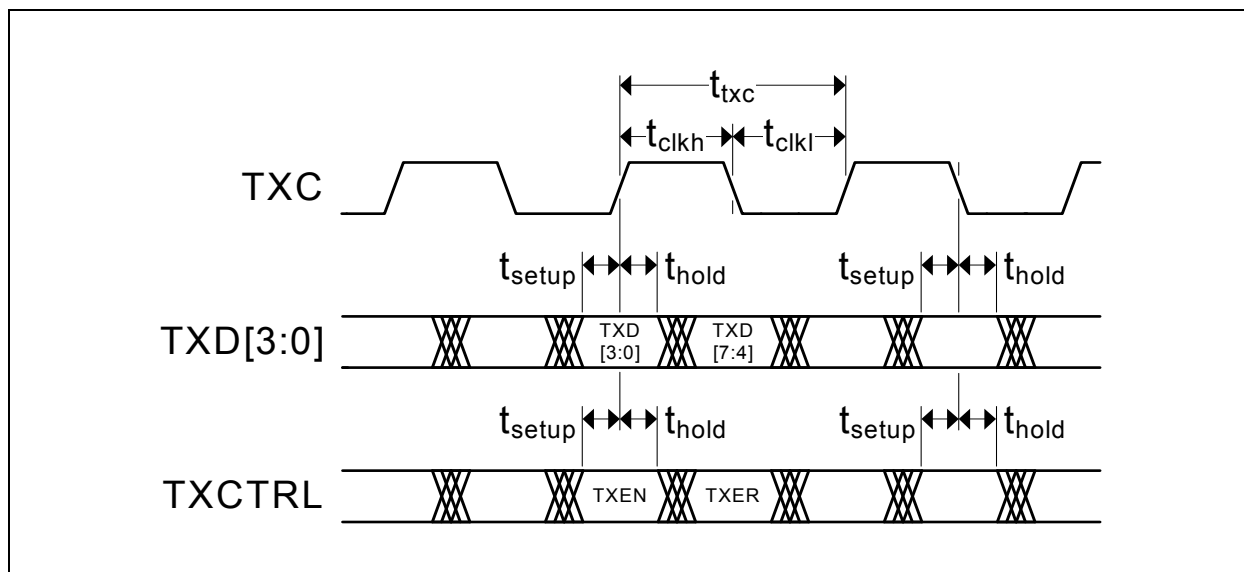
FIGURE 5-6: RGMII PHY TXC DELAY DISABLED TIMING
