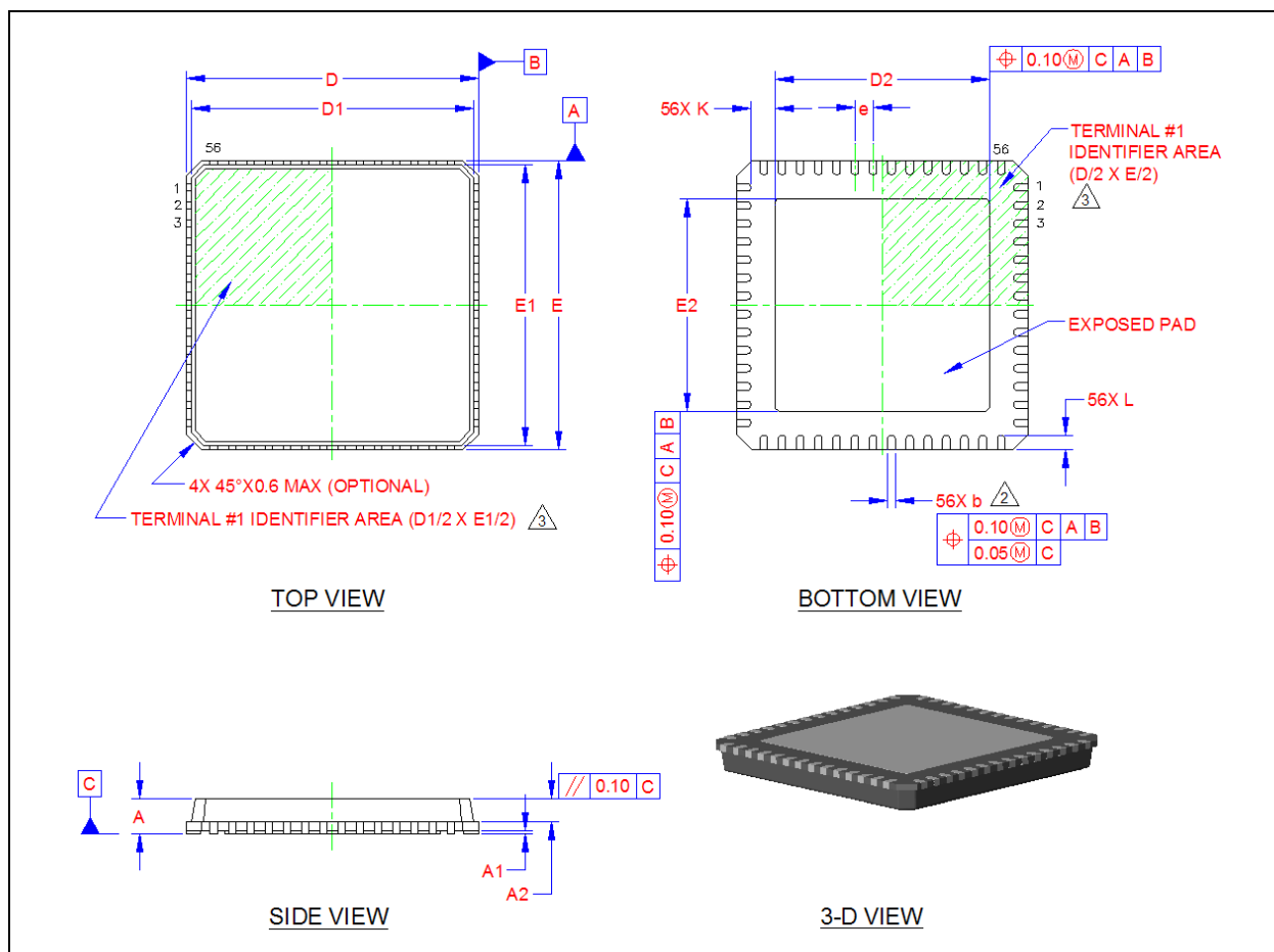
FIGURE 6-1: 56-QFN PACKAGE
