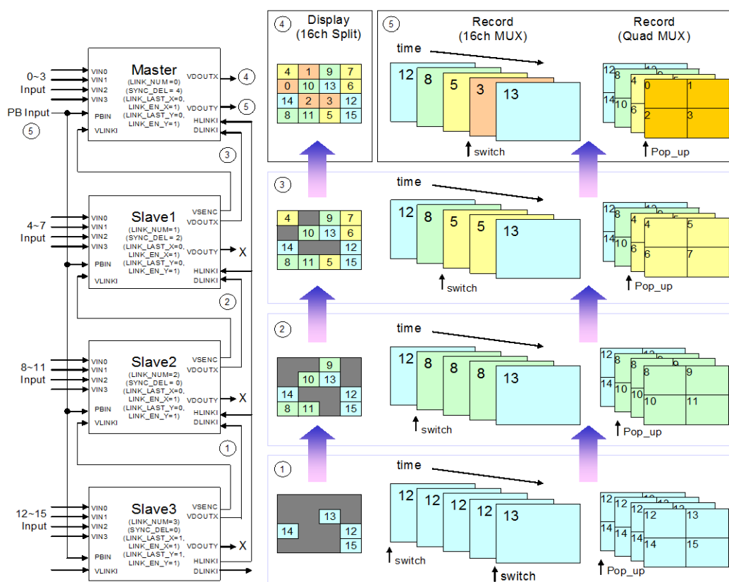
FIGURE 48 THE CASCADE CONNECTION FOR 120 CIE/SEC RECORD MODE
