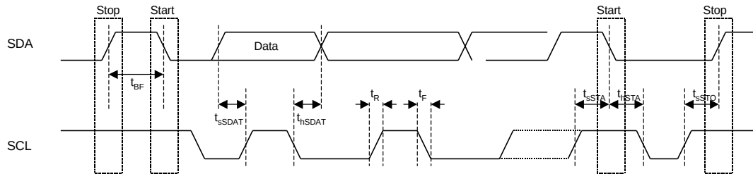
FIGURE 82 SERIAL INTERFACE TIMING DIAGRAM
