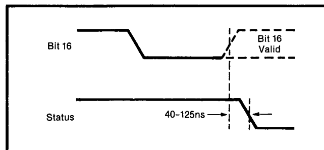
FIGURE 4. Timing Relationship of Valid Data to Status.
