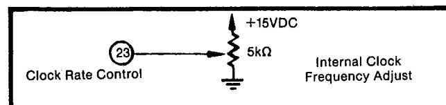
FIGURE 12. Clock Rate Control, Optional Fine Adjust.
