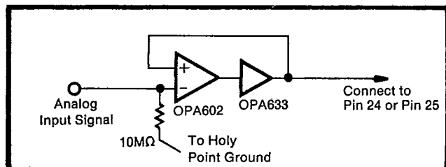
FIGURE 9. Source Impedance Buffering.
