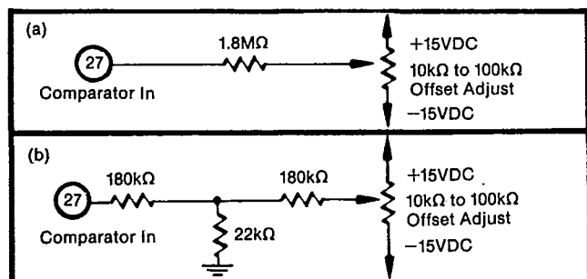
FIGURE 10. Two Methods of Connecting Optional Offset Adjust.
