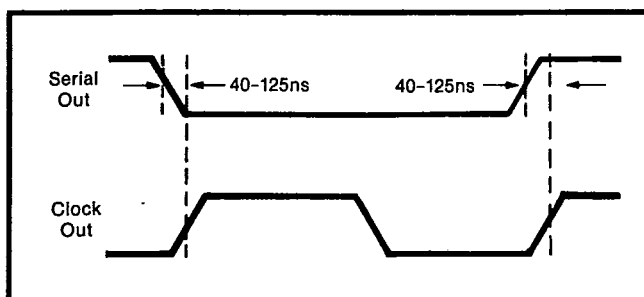
FIGURE 3. Timing Relationship of Serial Data to Clock.
