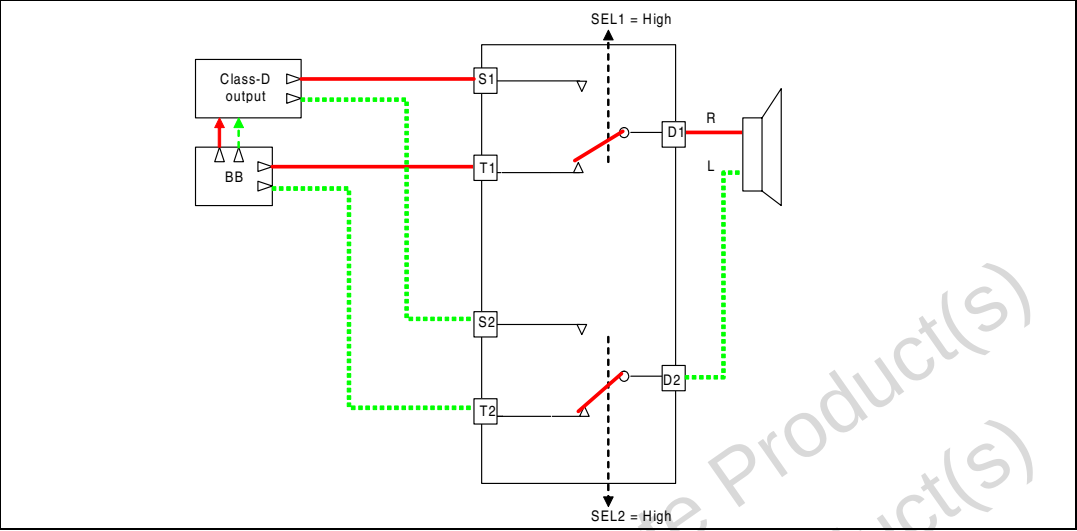
Figure 13. Application diagram
