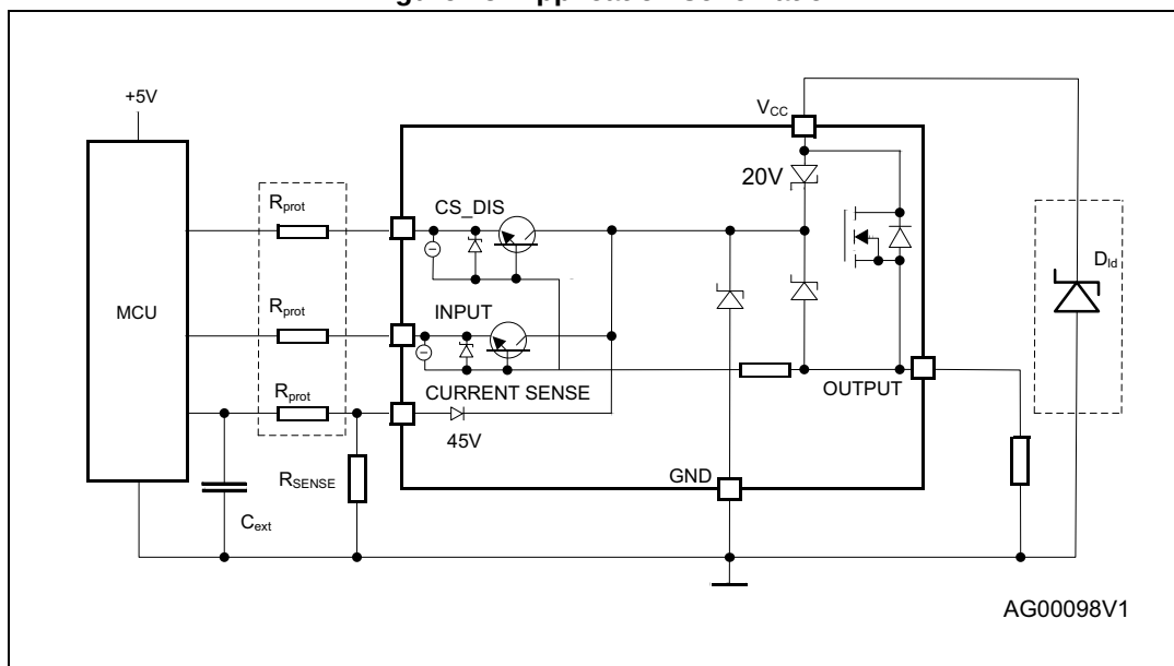
Figure 15. Application schematic
