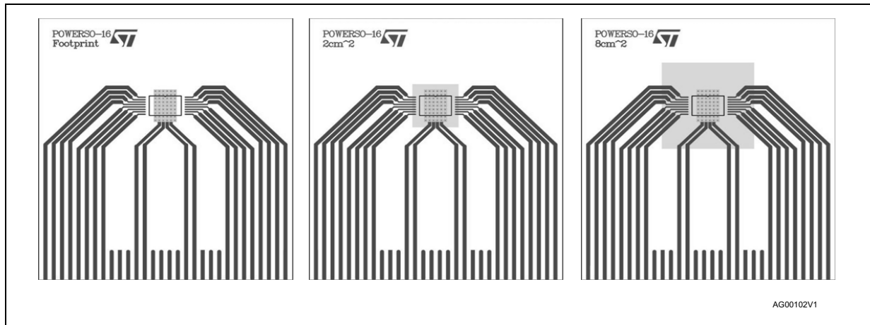
Figure 18. PowerSO-16 PC board
