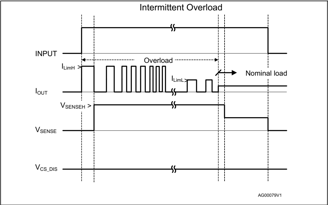
Figure 11. Intermittent overload
