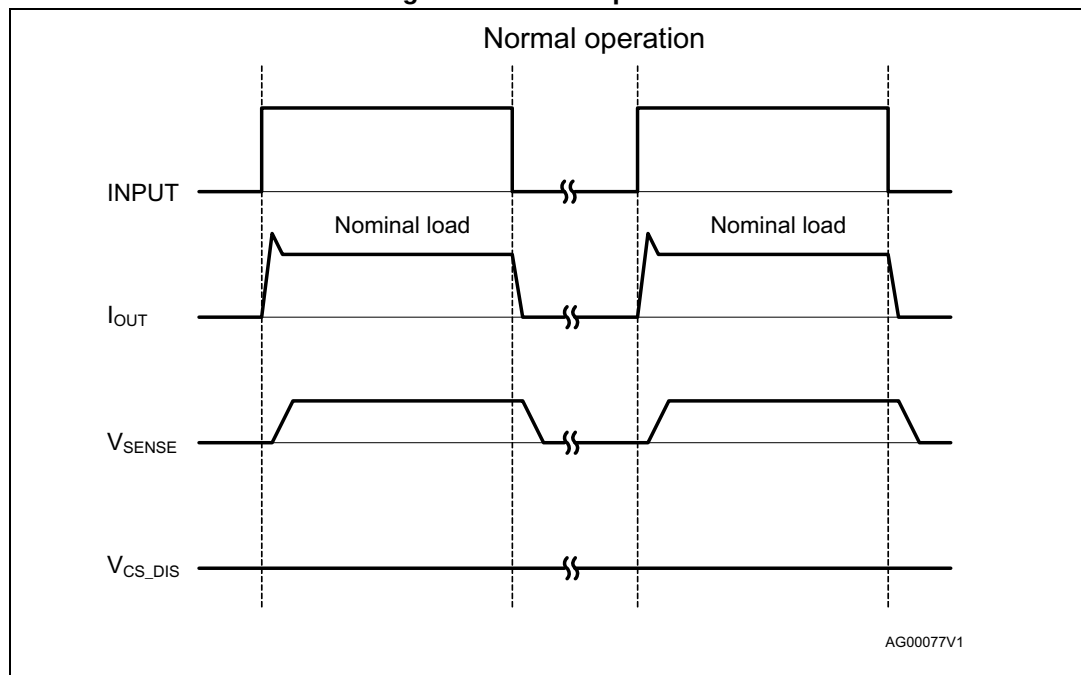
Figure 9. Normal operation
