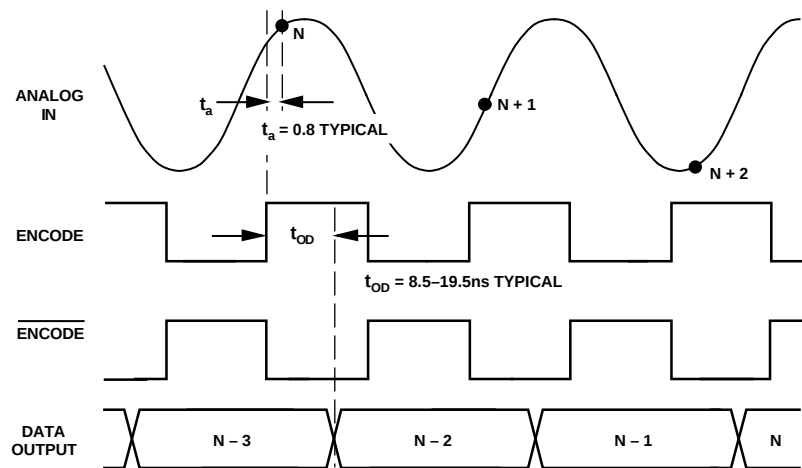
Timing Diagram
