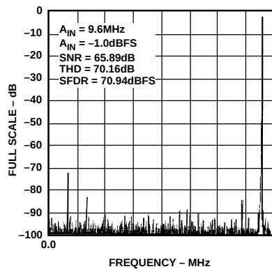
Figure 9. FFT Plot
