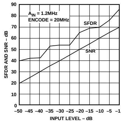
Figure 6. SFDR and SNR vs. Input Level
