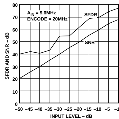
Figure 7. SFDR and SNR vs. Analog Input Level
