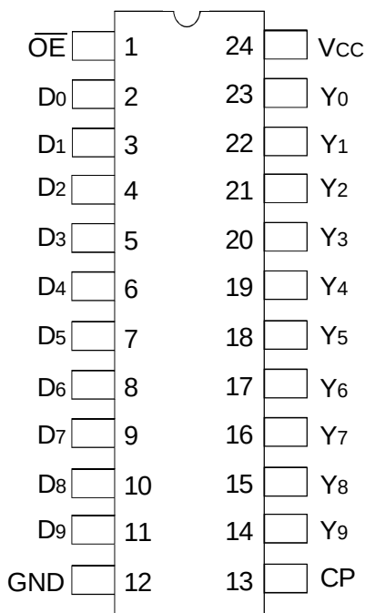
CERDIP/ SSOP/ QSOP TOP VIEW
