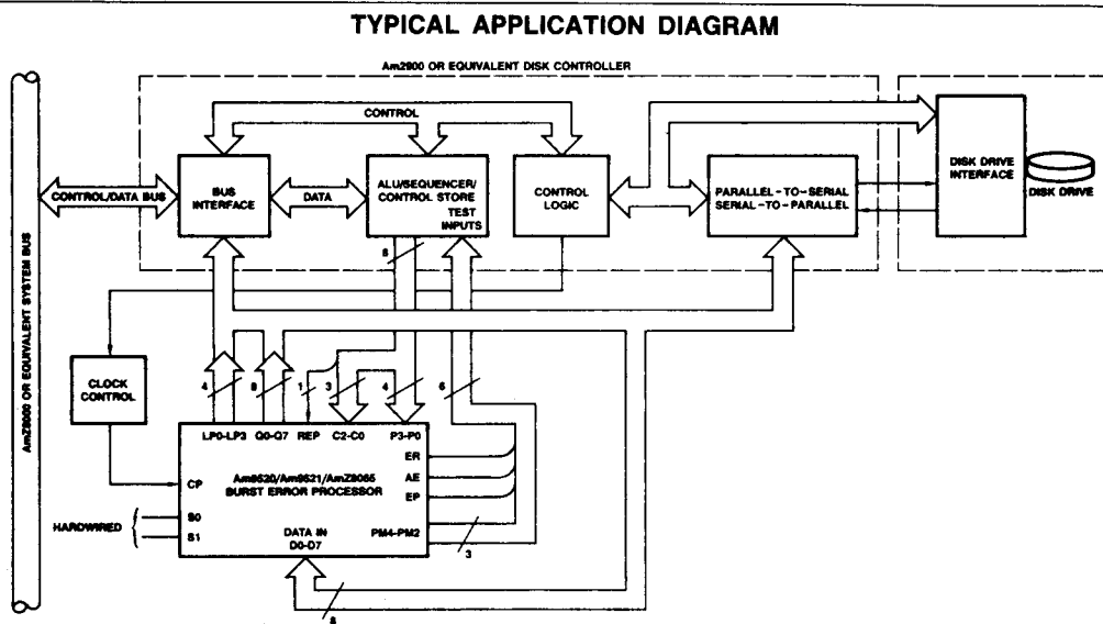
Figure 6. Am9520/Am9521/AmZ8065 Burst Error Processor
