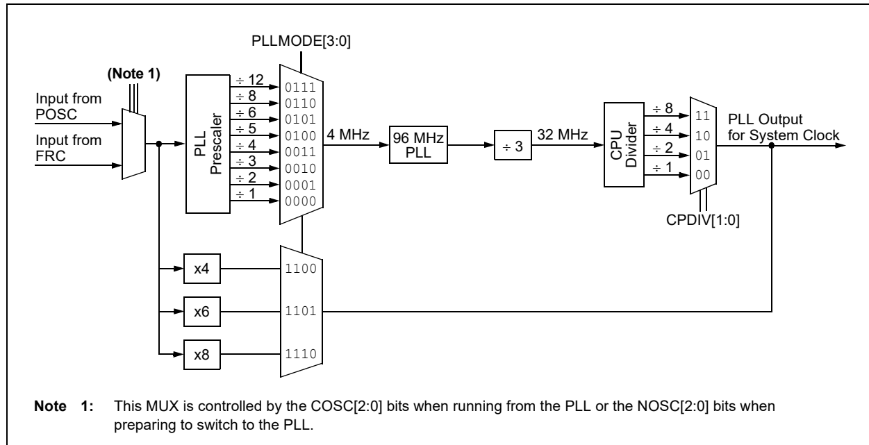
FIGURE 9-2: PLL BLOCK
