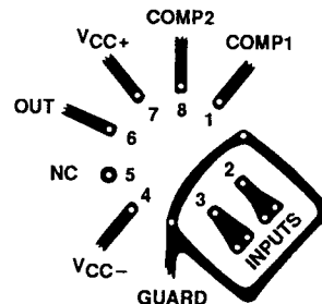
Figure 14. Input Guarding
