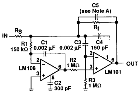
Figure 24. Amplifier for Photodiode Sensor
