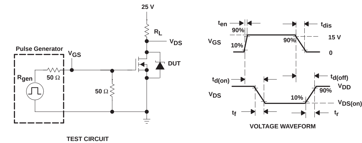
Figure 2. Resistive Switching
