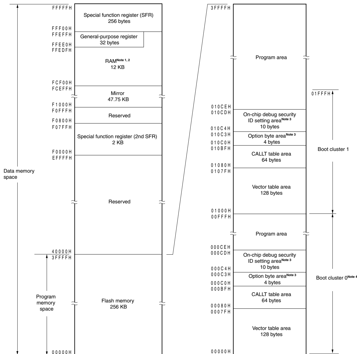
Figure 3-5. Memory Map (μPD78F1146, 78F1146A)
