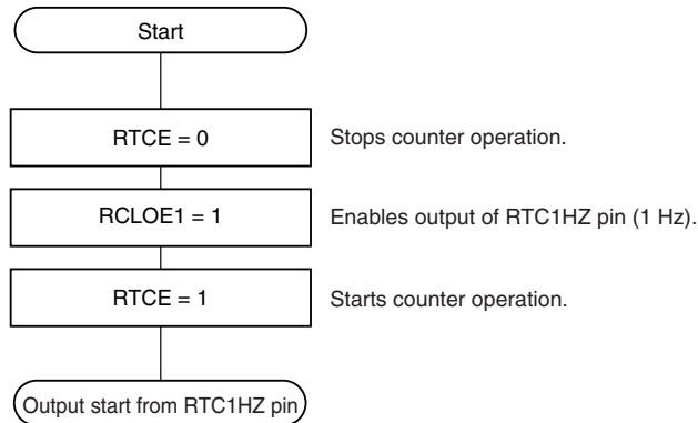
Figure 7-24. 1 Hz Output Setting Procedure
