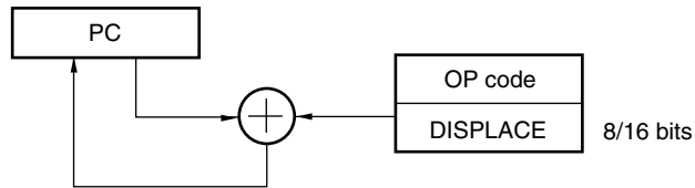
Figure 3-18. Outline of Relative Addressing
