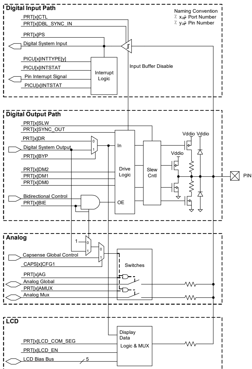
Figure 6-9. GPIO Block Diagram
