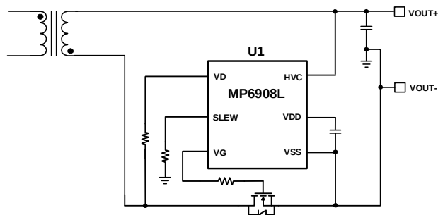
Figure 5: Low-Side Rectification
