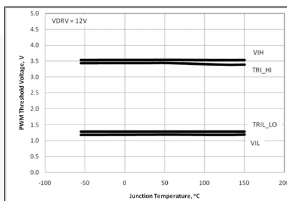
Figure 19. PWM Thresholds vs. Temperature
