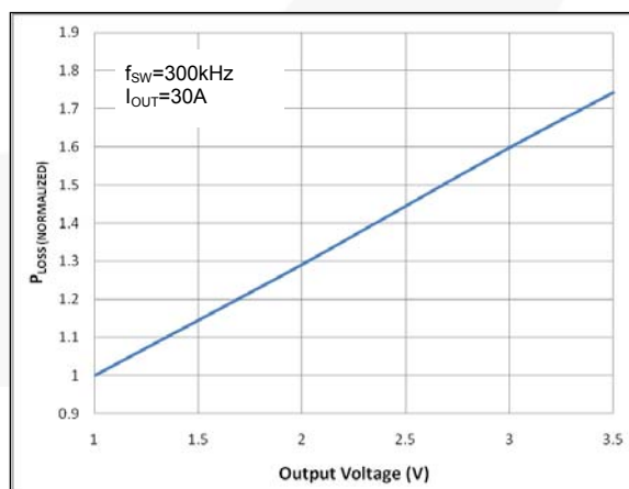
Figure 11. Power Loss vs. Output Voltage
