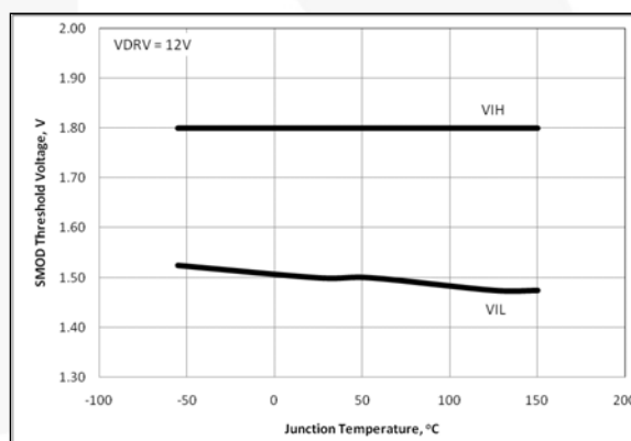
Figure 21. SMOD# Thresholds vs. Temperature
