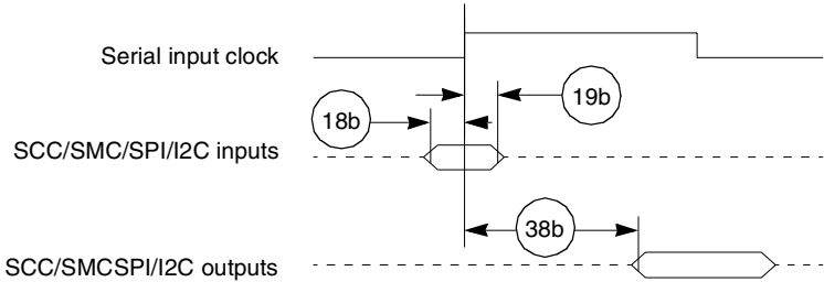
Figure 2-17. SCC/SMC/SPI/I 2 C External Clock Diagram
