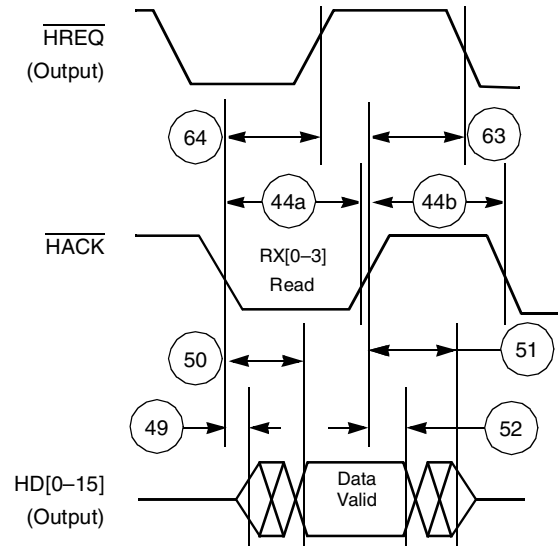
Figure 2-12. Host DMA Read Timing Diagram, HPCR[OAD] = 0
