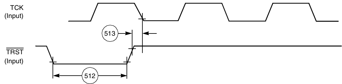
Figure 2-22. \overline{TRST} Timing Diagram
