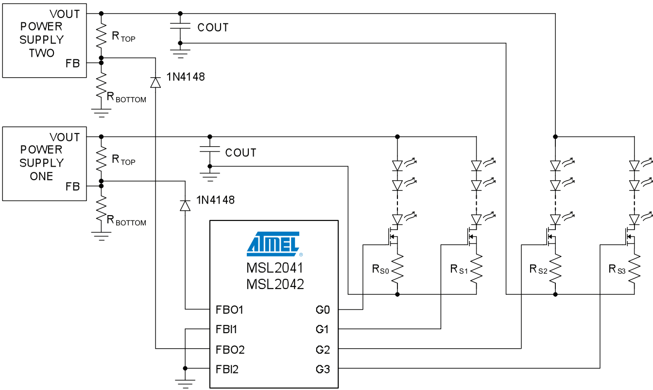
Figure 5. EO Configuration When Using Two String Power Supplies
