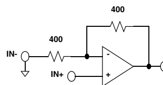
FIGURE 1. A_V = +2
