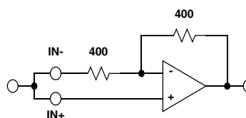
FIGURE 3. A_V = +1
