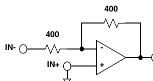
FIGURE 2. A_V = -1
