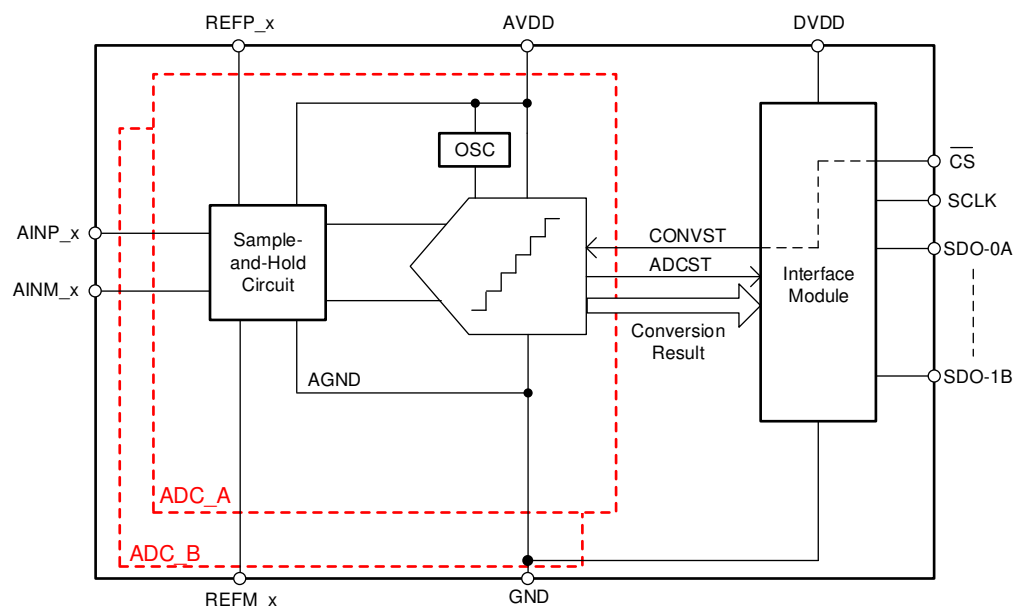
Figure 7-1. Converter Modules
