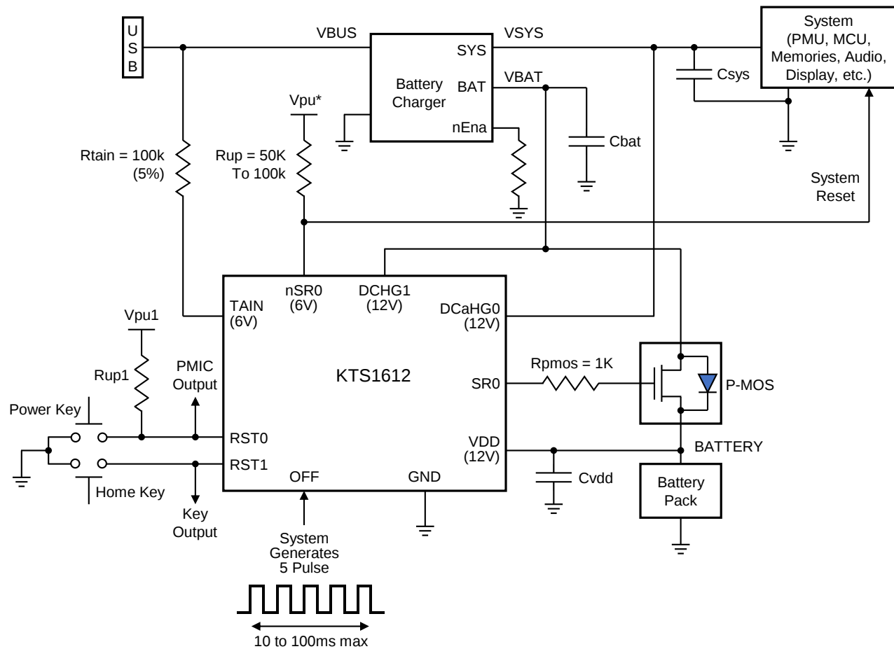
Figure 9. Application Circuit
