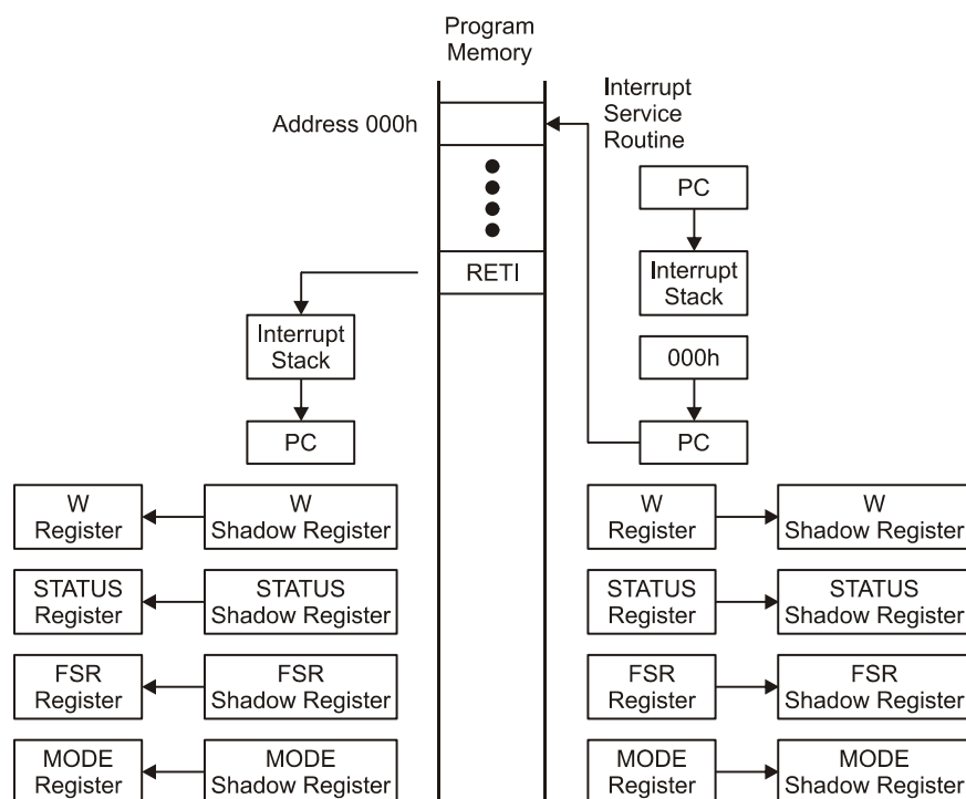
Figure 8-2: Interrupt Processing
