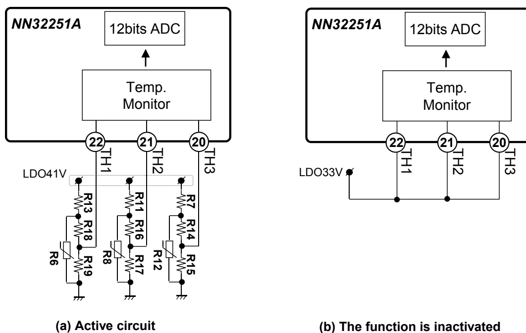
图A-5. Over-Temperature Detection
