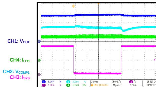
Load Transient
