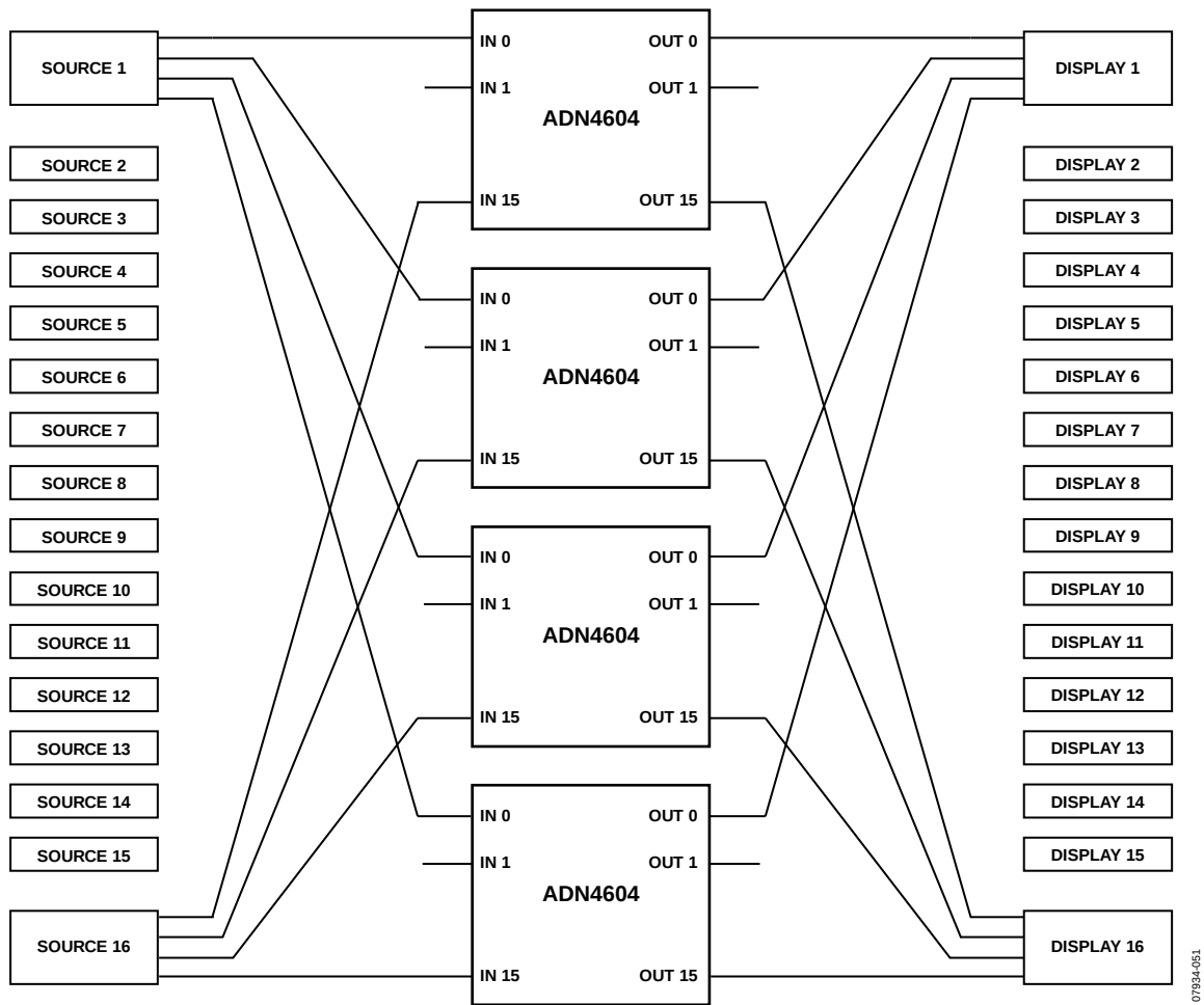
Figure 51. ADN4604 Digital Video (DVI, HDMI, DisplayPort) Matrix Switch Block Diagram
