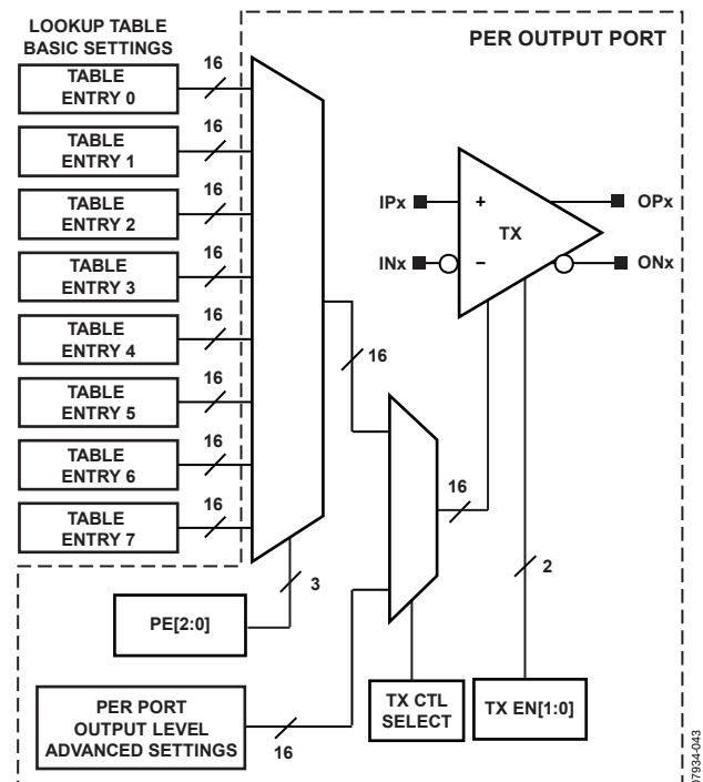
Figure 43. Transmitter Control Block Diagram
