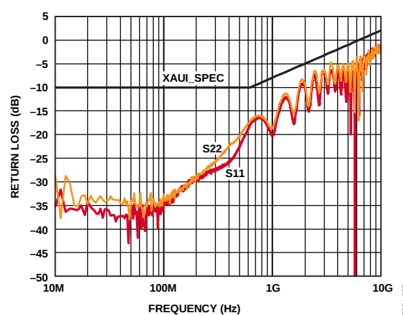
Figure 38. Return Loss (S11, S22)
