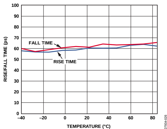
Figure 33. Rise/Fall Time vs. Temperature
