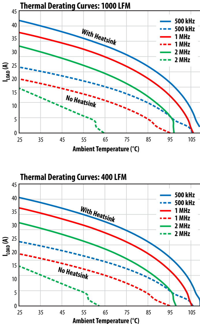
Figure 8: Thermal Derating Curves for Output Current Rating of EPC23103 IC using EPC90151 Evaluation Board
