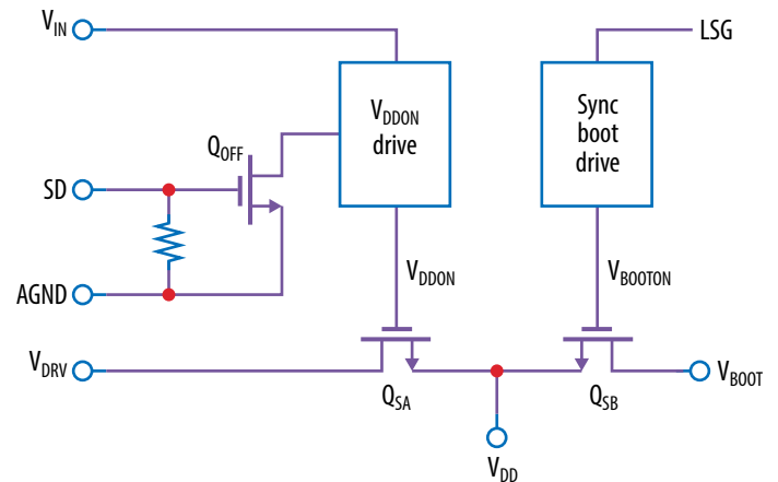
Figure 9: Simplified circuit diagram of V_{IN} , V_{DRV} , V_{DD} , and V_{BOOT} Power Supplies
