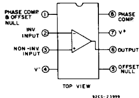
1g.—CA748CE and CA748E with external phase compensation.
