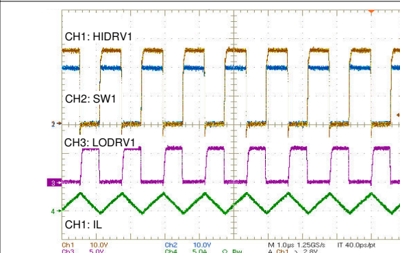
Figure 10-6. Line Regulation
