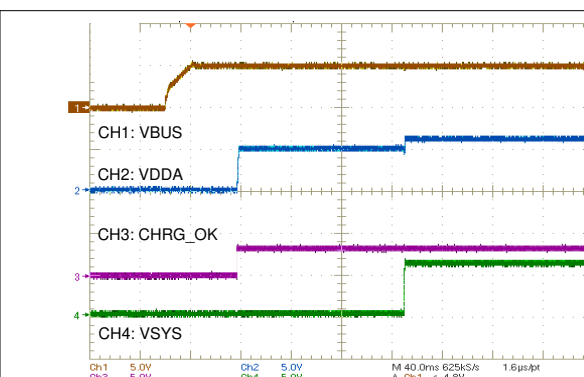
Figure 10-4. Power Up From 5 V
