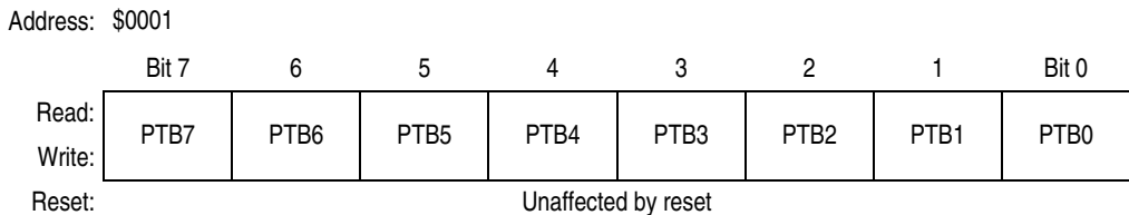
Figure 13-6. Port B Data Register (PTB)
