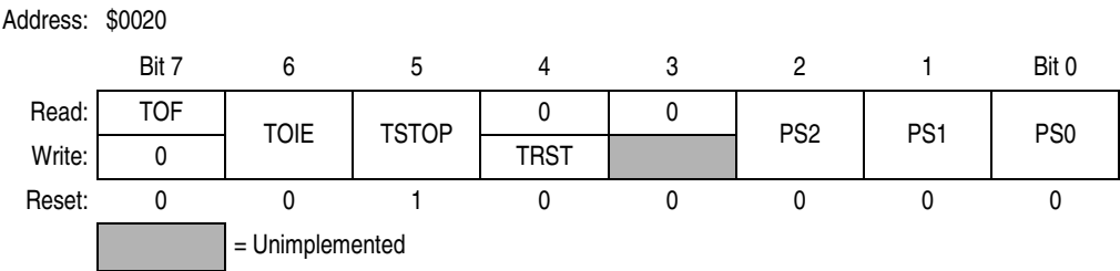
Figure 15-5. TIM Status and Control Register (TSC)
