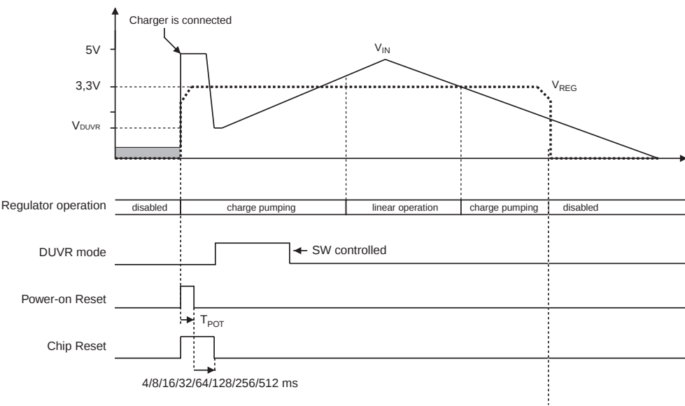
Figure 22-2. Voltage regulator operation and reset signals as a function of rising and falling input voltage for 1-cell operation.
