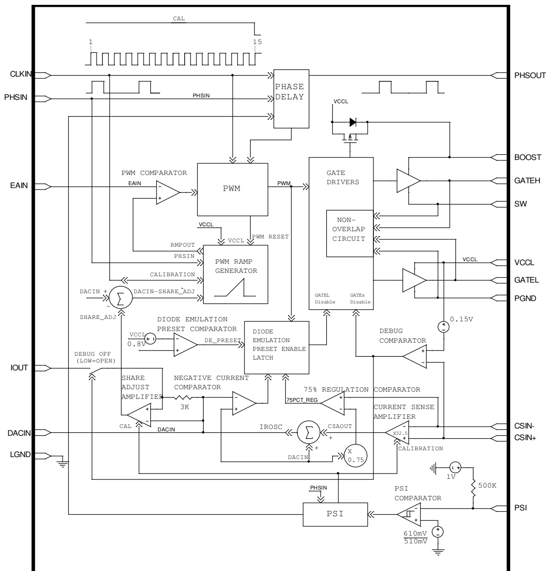
Figure 5 Block diagram
