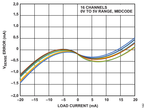
Figure 41. V_{SENSE} Error vs. Load Current from Equation 5
