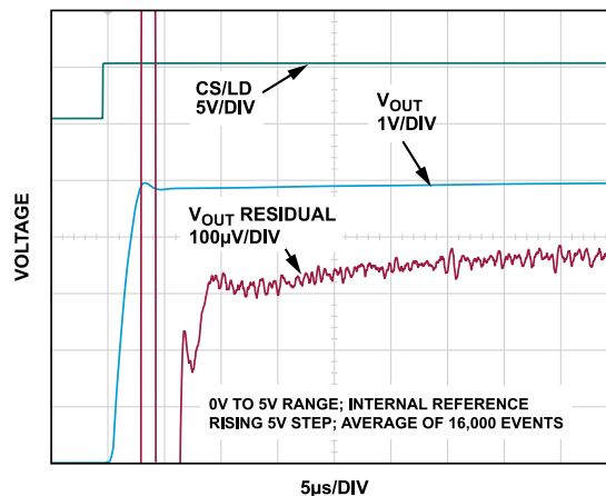
Figure 31. Settling Time, 5 V
