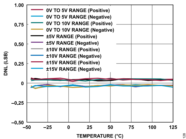
Figure 28. DNL vs. Temperature
