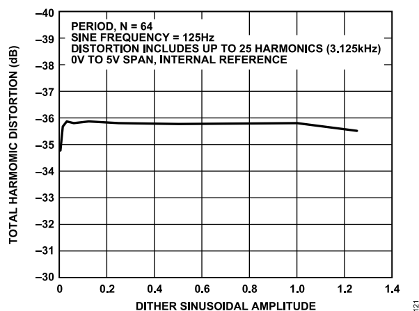
Figure 21. Total Harmonic Distortion (THD) vs. Dither Sinusoidal Amplitude
