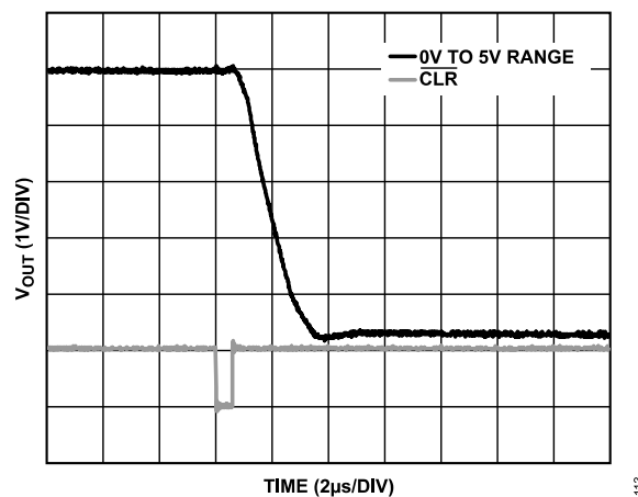
Figure 13. Hardware \overline{CLR} to Zero Scale
