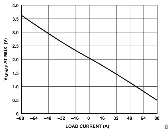
Figure 20. V_{SENSE} at MUX vs. Load Current
