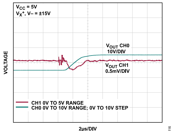
Figure 16. DAC to DAC Crosstalk
