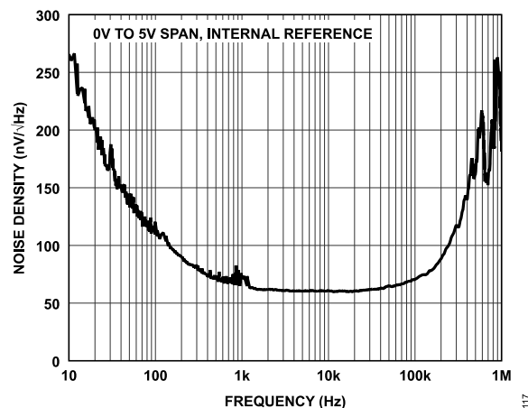
Figure 17. Noise Density vs. Frequency
