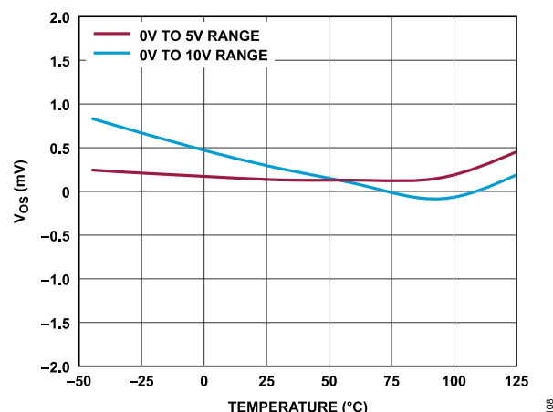
Figure 8. Unipolar Offset Error ( V_{OS} ) vs. Temperature
