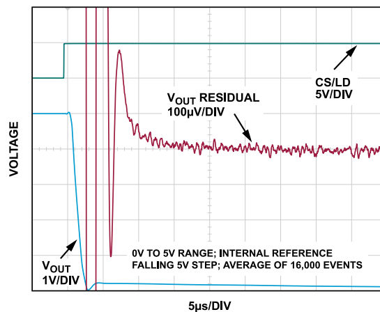
Figure 32. Settling Time, 5 V (Falling)
