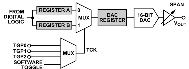
Figure 47. Toggle Operation
