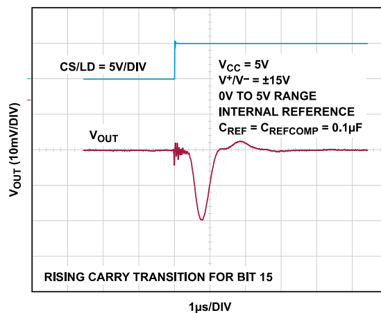
Figure 15. Glitch Impulse
