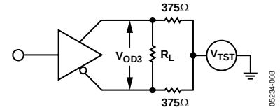
Figure 8. Driver Voltage Measurement Test Circuit 2
