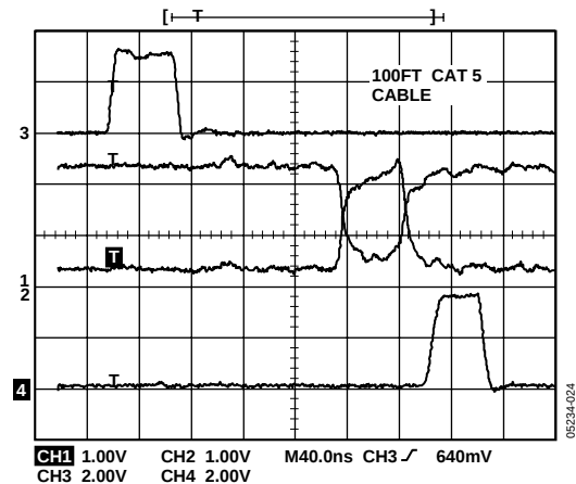
Figure 24. Driving 100 ft. Cable H-L Transition
