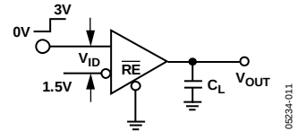
Figure 11. Receiver Propagation Delay Test Circuit
