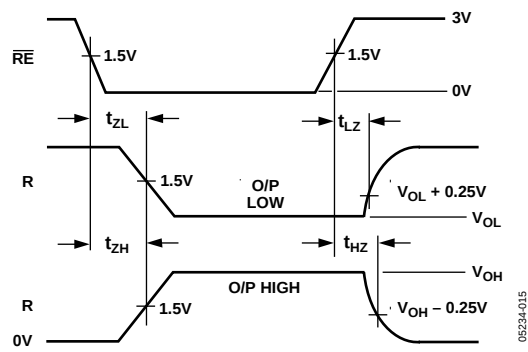
Figure 15. Receiver Enable/Disable Timing
