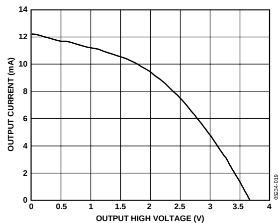
Figure 19. Receiver Output High Voltage vs. Output Current
