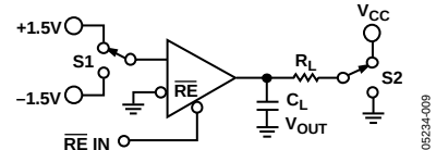
Figure 9. Receiver Enable/Disable Test Circuit
