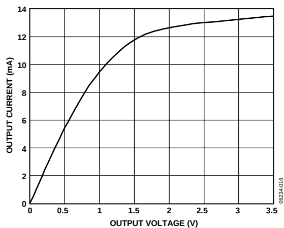
Figure 16. Receiver Output Low Voltage vs. Output Current
