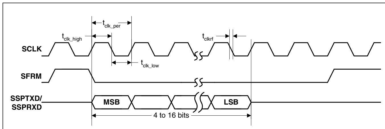
Figure 18. TI Single Transfer Timing Measurement
