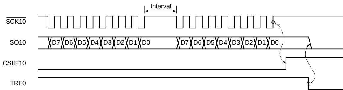
Figure 12-10. Basic Transmit Mode Operation Timing
