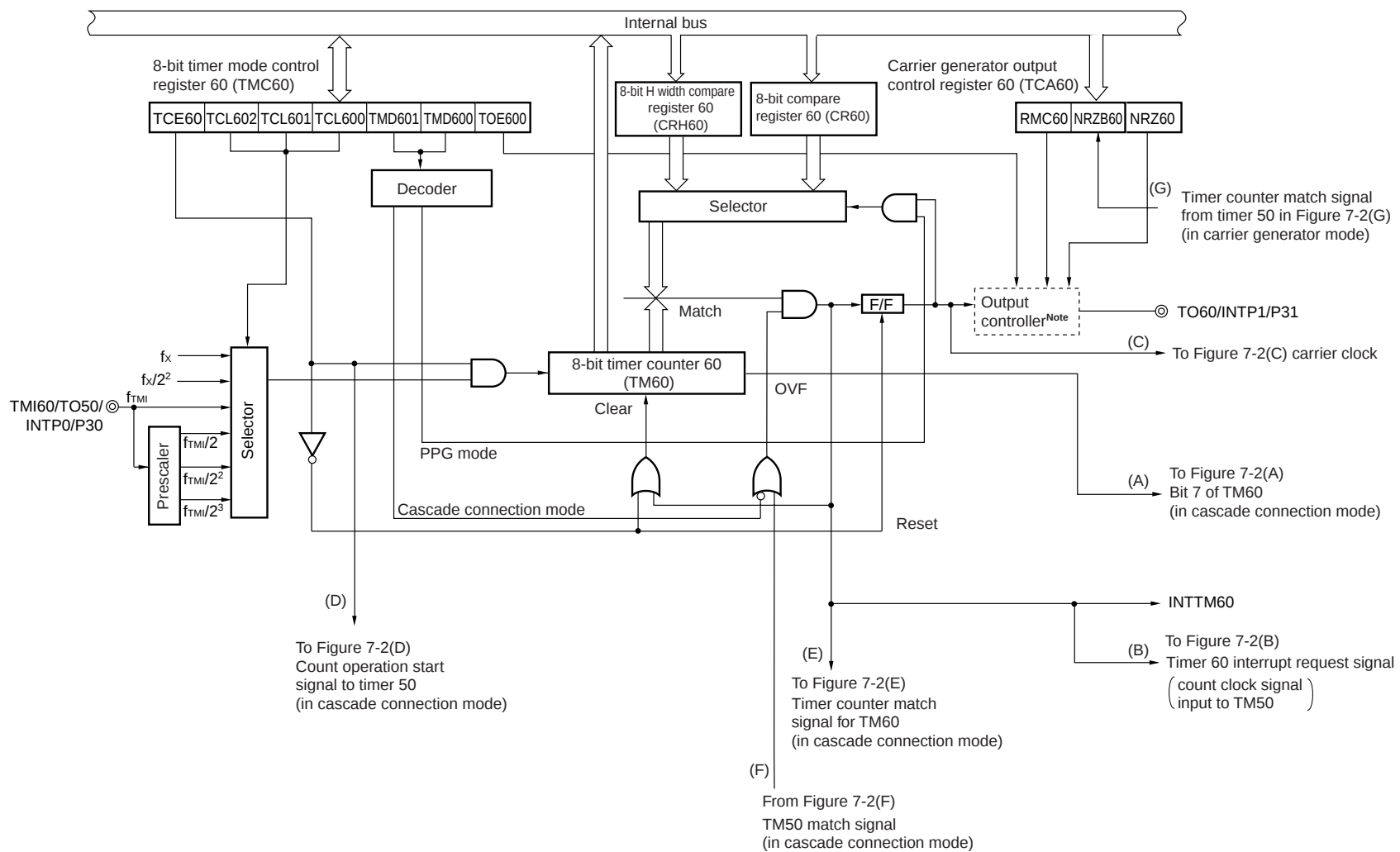
Figure 7-3. Block Diagram of Timer 60
