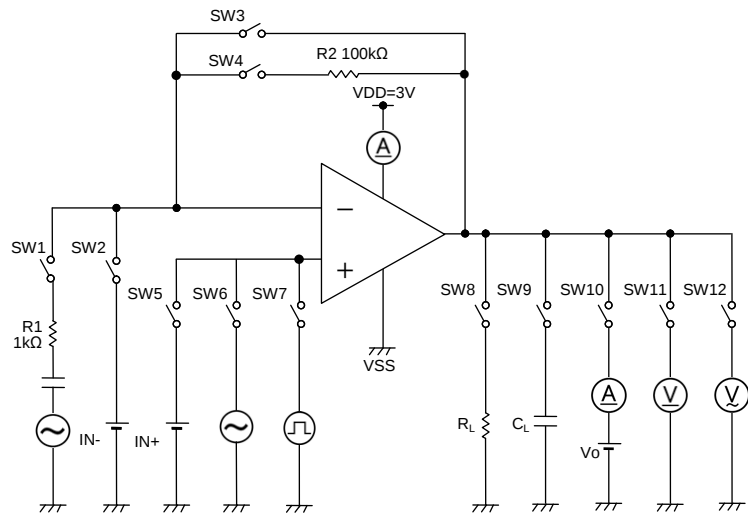
Figure 25. Test Circuit 2
