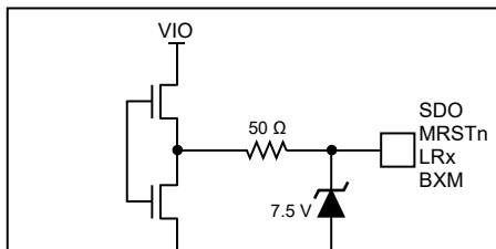
Figure 17h: Logic Outputs
