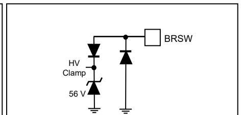
Figure 17i: HV-Compliant BRSW Output
