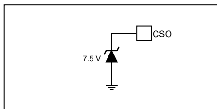
Figure 17k: Current Sense Amp Output
