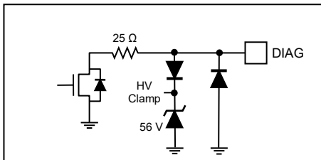
Figure 17g: HV-Compliant DIAG Output
