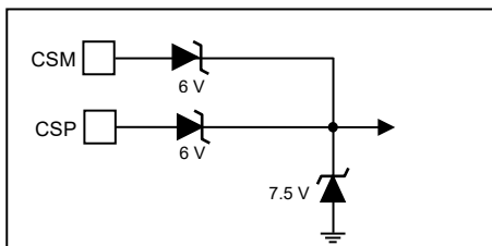
Figure 17j: Current Sense Amp Inputs
