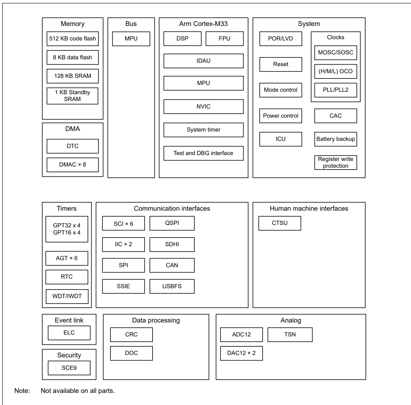
Figure 1.1 Block diagram
