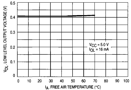
Figure 8. Low Level Output Voltage versus Temperature
