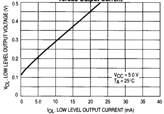
Figure 6. Low Level Output Voltage versus Output Current
