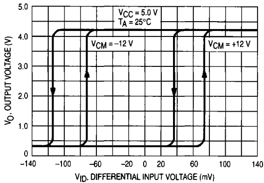
Figure 3. Output Voltage versus Differential Input Voltage
