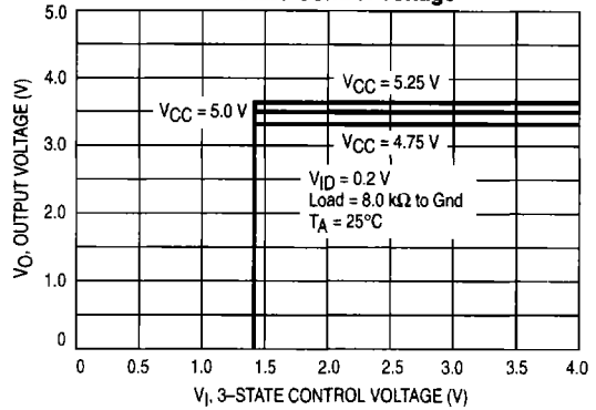
Figure 4. Output Voltage versus 3-State Control Voltage
