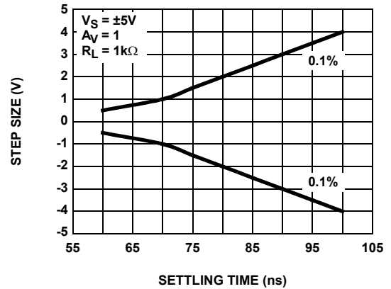
FIGURE 24. SETTLING TIME vs STEP SIZE
