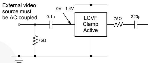
Figure 19. Biased SCART with AC-Coupled Outputs
