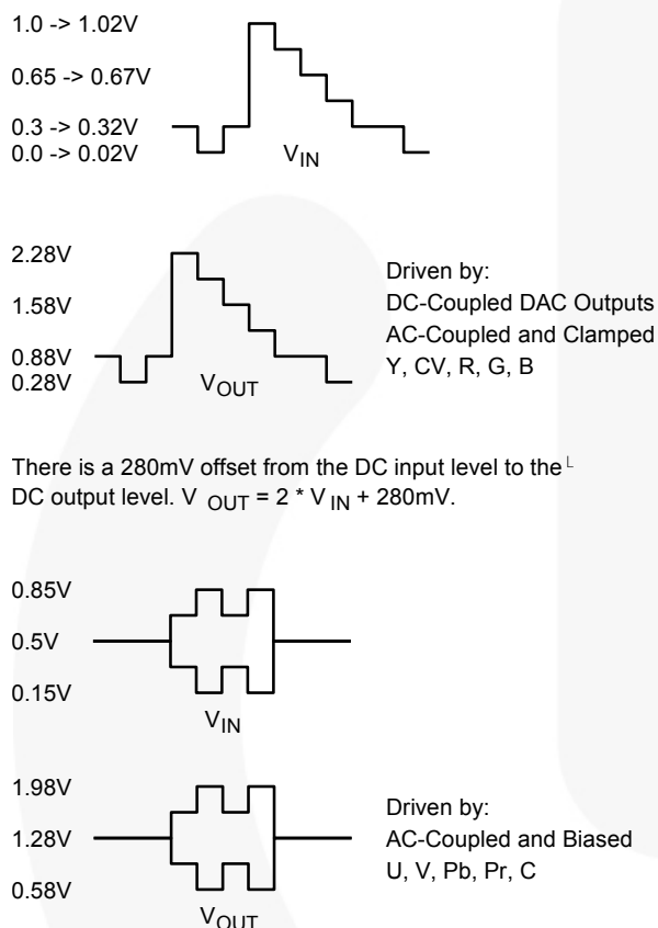
Figure 11. Typical Voltage Levels
