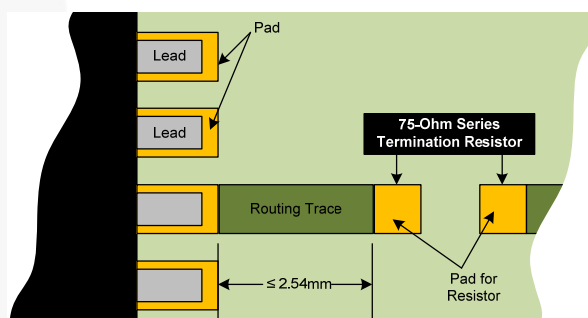
Figure 20. Termination Resistor Placement
