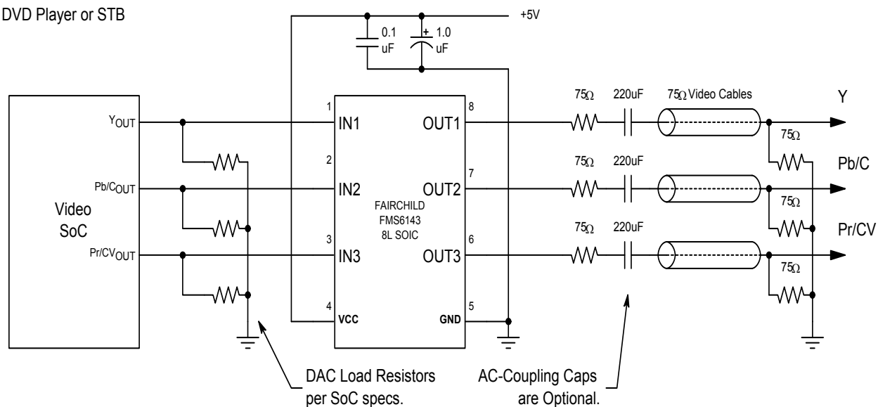
Figure 10. Typical Application
