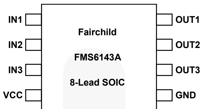
Figure 2. Pin Assignments
