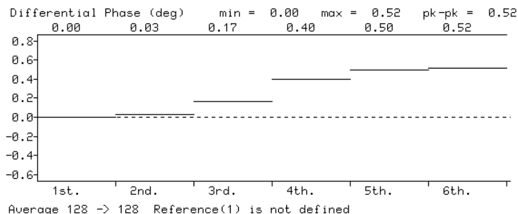
Figure 8. Differential Phase
