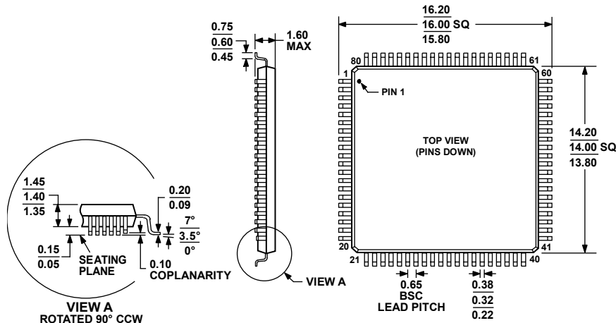
COMPLIANT TO JEDEC STANDARDS MS-026-BEC Figure 36. 80-Lead Low Profile Quad Flat Package [LQFP] (ST-80-2) Dimensions shown in millimeters
