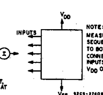
Fig. 20—Input leakage current test circuit.
