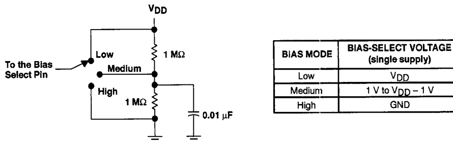
Figure 1. Bias Selection for Single-Supply Applications
