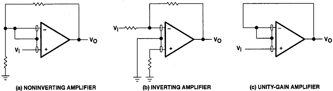
Figure 107. Guard-Ring Schemes
