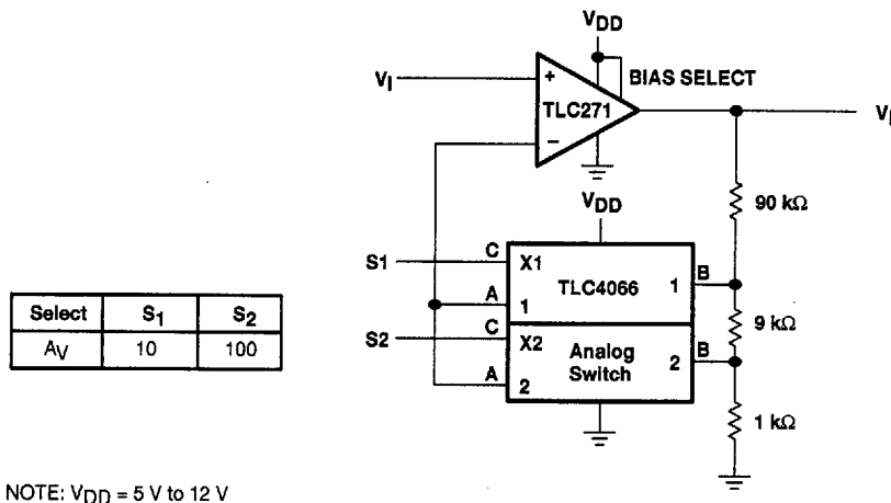
Figure 125. Amplifier With Digital Gain Selection
