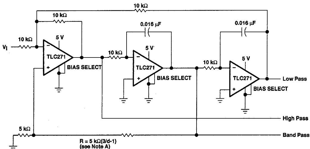
Figure 114. State-Variable Filter
