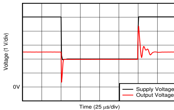
Figure 6-26. Supply Transient Response, A5 devices
