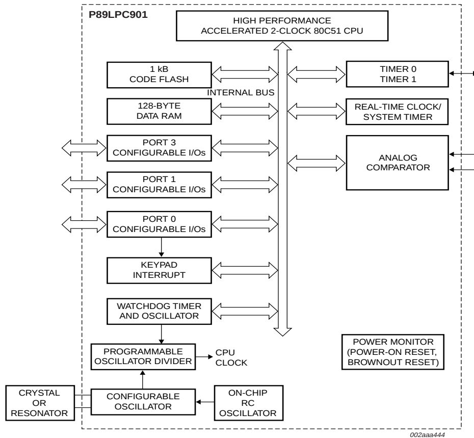
Fig 1. P89LPC901 block diagram.
